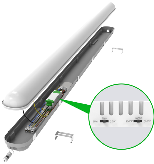
CCT & wattage switches on the driver
